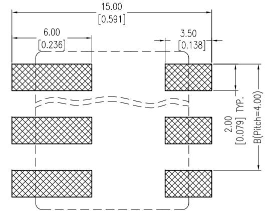
Recommended P.C.B Layout(Top Side) (PCB BOARD TOLERANCE±0.05)
