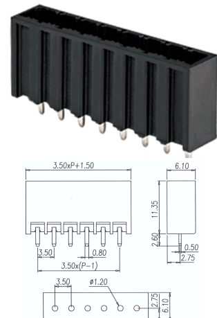
P/N: BC022537-XX-TH
