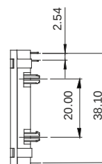
RECOMMENDED HOLE PATTERN
