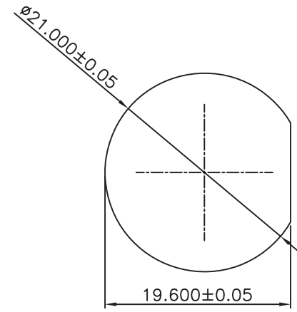
Panel Cut-Out Panel Thick: 1.5~2.0mm
