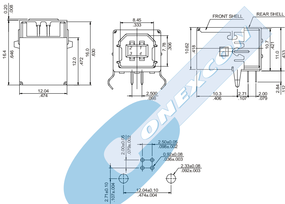
RECOMMENDED HOLE PATTERN
