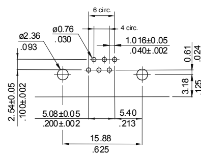
RECOMMENDED HOLE PATTERN
