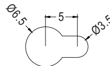
MOUNTING HOLE
