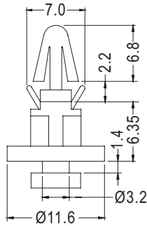
MOUNTING HOLE
