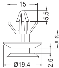
MOUNTING HOLE
