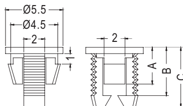
CHASSIS Ø4.5
