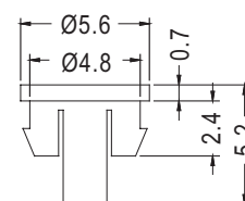
CHASSIS Ø5.0 THICKNESS 1.0~1.1
