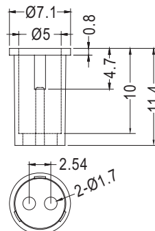
CHASSIS Ø6.35 THICKNESS 0.8~1.4
