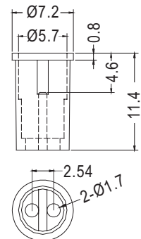
CHASSIS Ø6.4 THICKNESS 0.8~1.4
