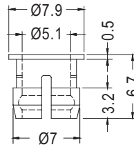
FOR LED5-2A
