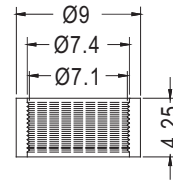
FOR LED5-2B
