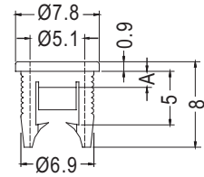
CHASSIS Ø7.0 THICKNESS A
