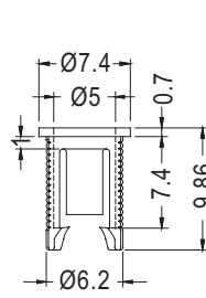
CHASSIS Ø6.35
