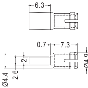
CHASSIS Ø4.4 THICKNESS 1.57~3.2
