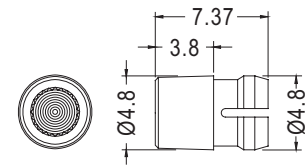
CHASSIS Ø4.4 THICKNESS 1.57~3.2
