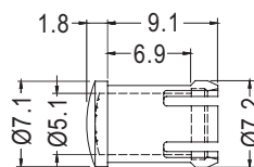
CHASSIS Ø6.4 THICKNESS 0.8~6.35
