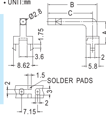
PCB LAYOUT.
