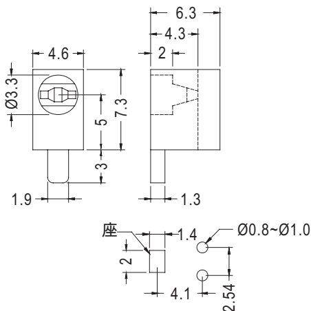
MOUNTING HOLE
