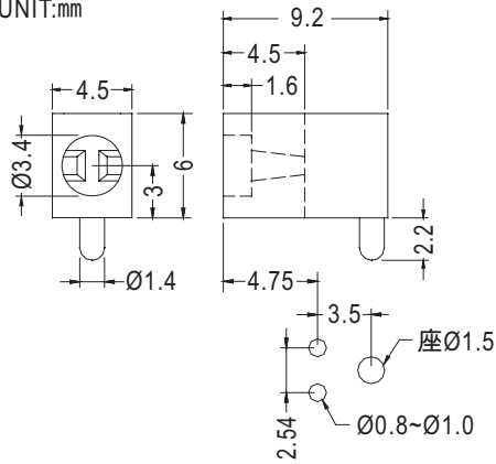
MOUNTING HOLE
