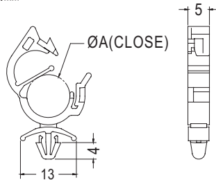
CHASSIS Ø4.0 THICKNESS 0.8~1.6
