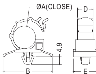
CHASSIS Ø6.4 THICKNESS : C
