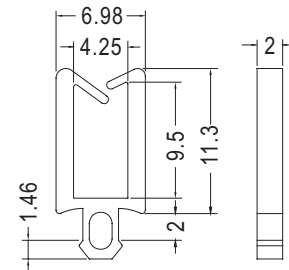
P.C.B Ø2.8 THICKNESS 2.0
