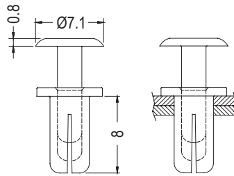
CHASSIS Ø4.0 THICKNESS 5.5~6.5
