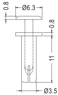
CHASSIS Ø3.5
