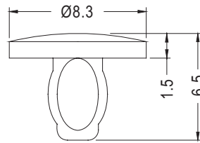
CHASSIS Ø3.2~Ø3.5
