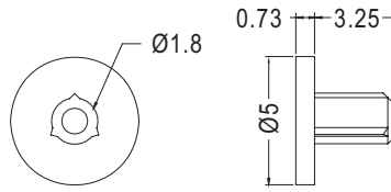
CHASSIS Ø1.8~Ø2.0
